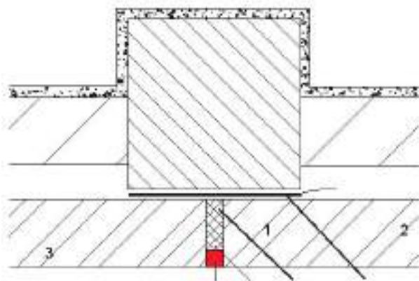
Example of brickwork expansion joint
