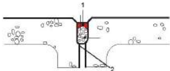
1 Nitoseal MS100 2 Expandable foam cord
